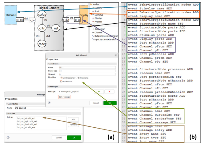
Fig. 1. HEPHYCODE Graphical Modeling Workbench (a) and trace file generated through MER tool (b). The application considered in this scenario is called Digital Camera [9].
