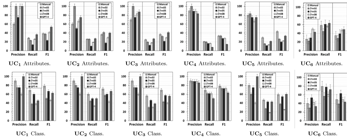
Fig. 11. Validation results for the considered MSEs on dataset D_3 for the different dataset D_1 (Manual, D2 (GPT4), Dm02, Dm05, and Dm08 (Mixed)).
