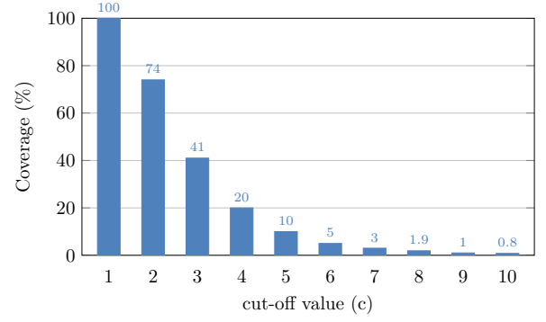
Figure 3. Distribution of the number of topics in the dataset. the prediction of more than 5 featured topics becomes a hard task considering this strict assumption.
